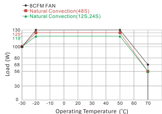
ARF130O Series Vin at 230-264 VAC
