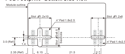
PCB Footprint - Bottom Side View
