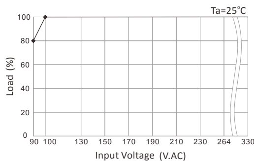
ATCW40 Series Derating Load versus Input Voltage
