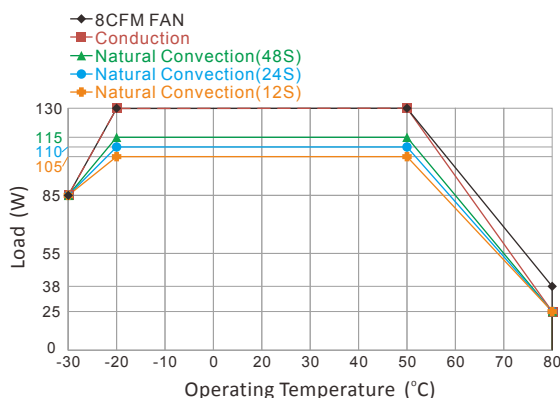
ARF130E Series Vin at 100-114 VAC
