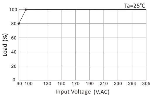
AHCH10 / AOCK10 Series Derating Load versus Input Voltage
