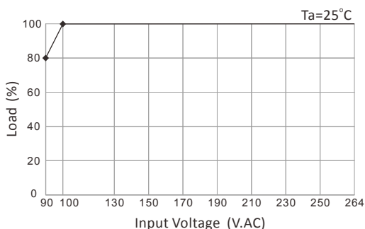
SZA60 Series Derating Load versus Input Voltage
