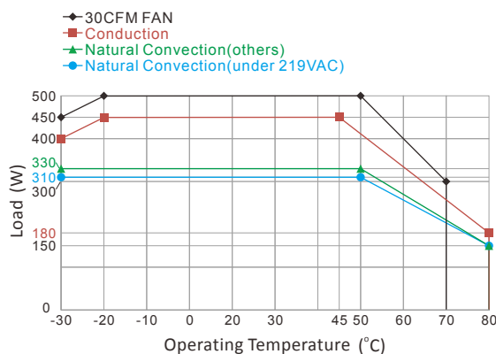
ARF500U Series Vin at 198-264 VAC
