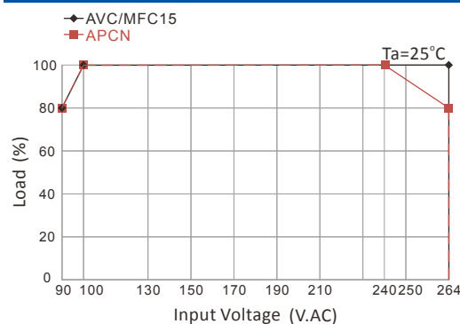
Derating Load versus Input Voltage
