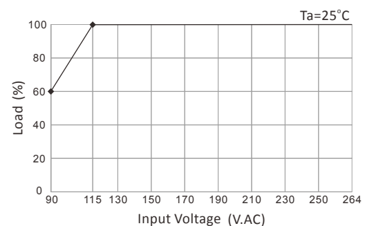
MQF500 Series Derating Load versus Input Voltage
