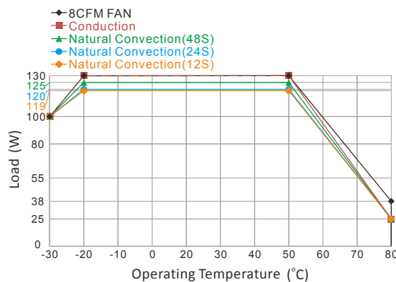
ARF130U / AQF130E Series Vin at 115-264 VAC
